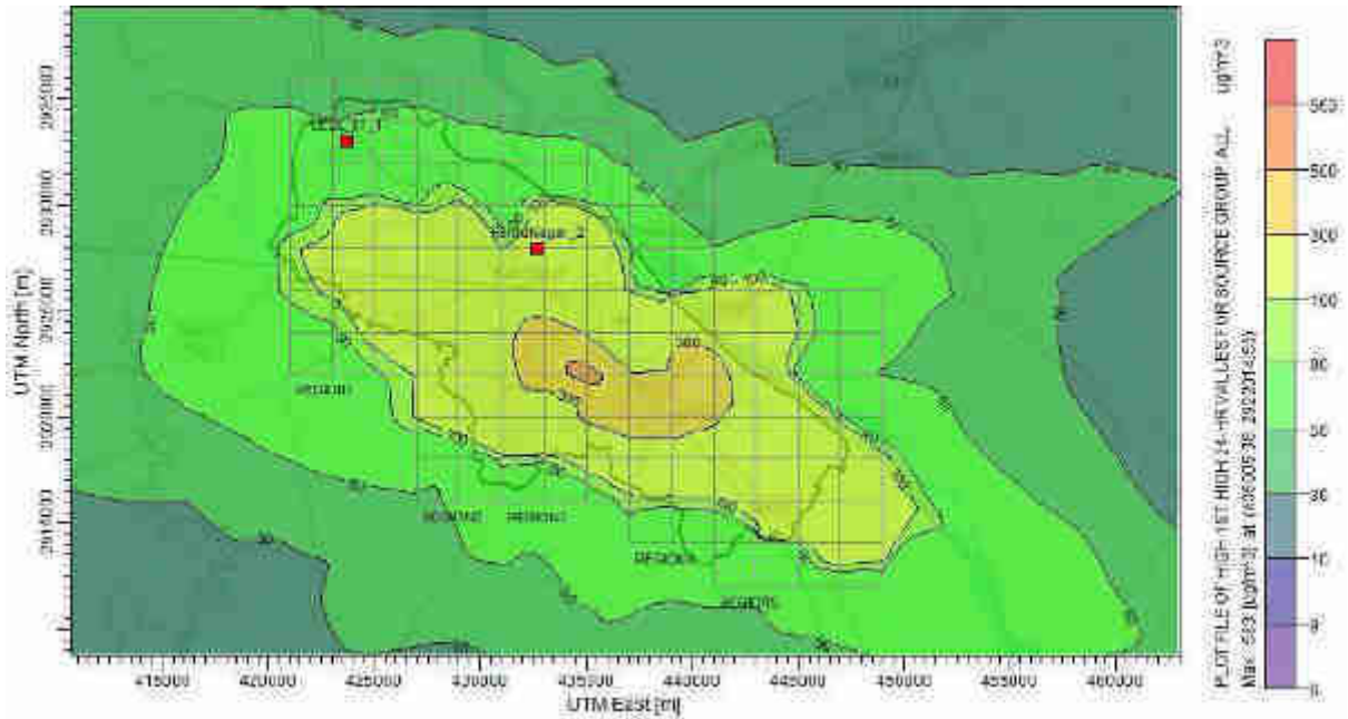
Figure 5.21: Highest 24-hour Average PM 2.5 Levels from All Sources (Scenarios 1)
