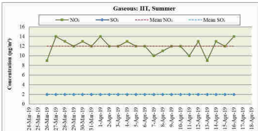
Figure 2.55: SO 2 and NO 2 Concentrations at IIT for Summer Season
