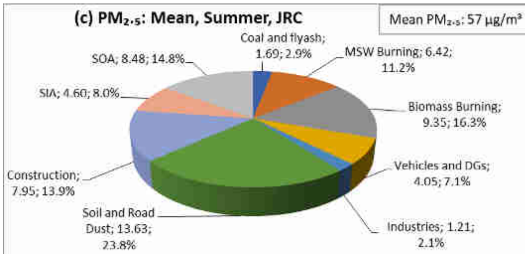
Figure 4.25: PMF modeling for PM 2.5 at JRC for summer season
