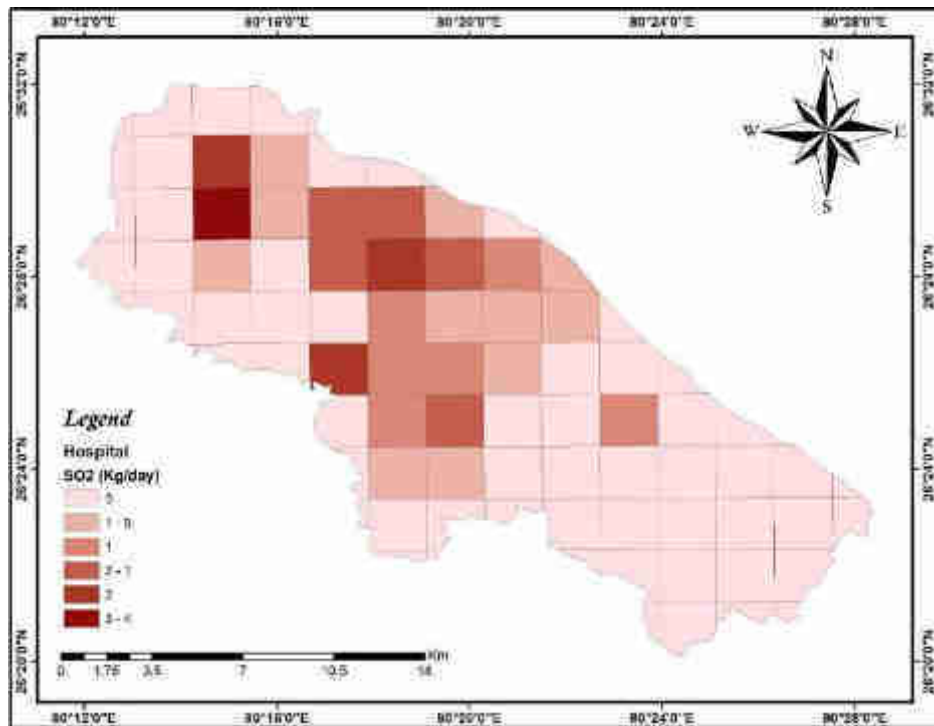
Figure 3.61: Spatial Distribution of SO 2 Emissions from Hospitals
