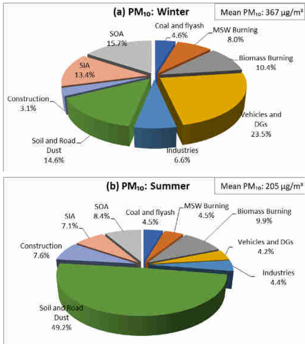
Figure 4.35: Overall source contribution to PM 10 in (a) winter and (b) summer
