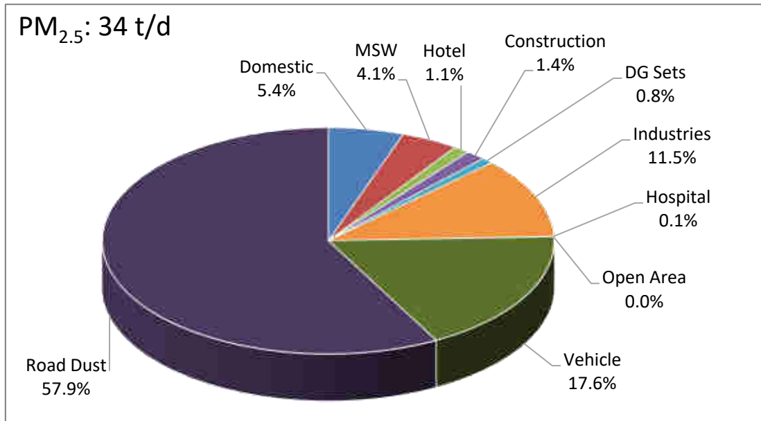
Figure 3.105: PM 2.5 Emission Load of Different Sources
