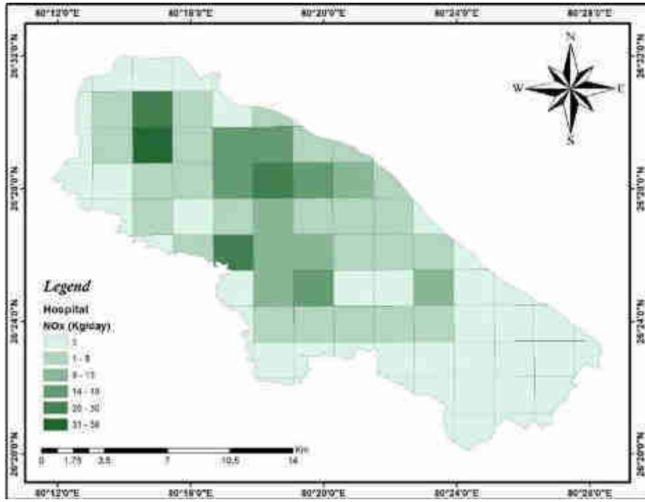
Figure 3.60: Spatial Distribution of NO x Emissions from Hospitals
