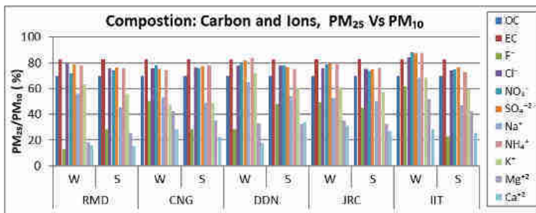
Figure 2.76: Compositional comparison of carbon and ions species in PM 2.5 Vs PM 10
