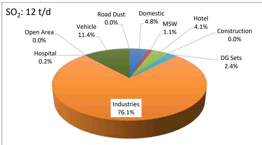
Figure 3.106: SO 2 Emission Load of Different Sources
