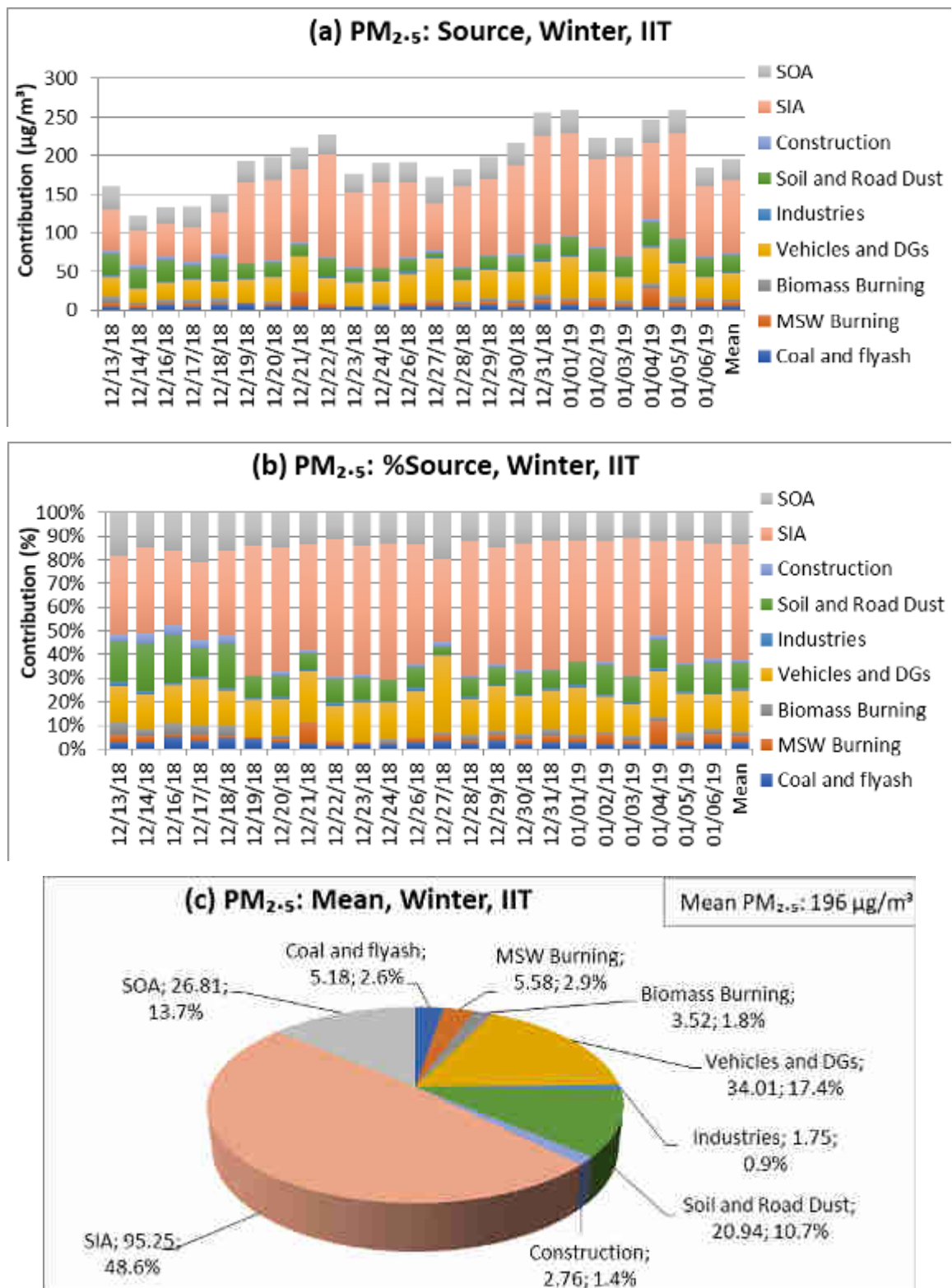
Figure 4.28: PMF modeling for PM 2.5 at IIT for winter season
