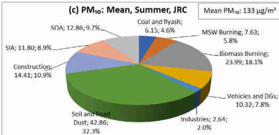
Figure 4.24: PMF modeling for PM 10 at JRC for summer season
