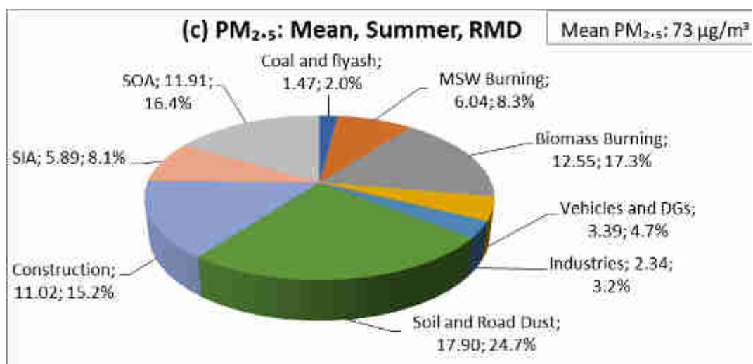
Figure 4.7: PMF modeling for PM 2.5 at RMD for summer season
