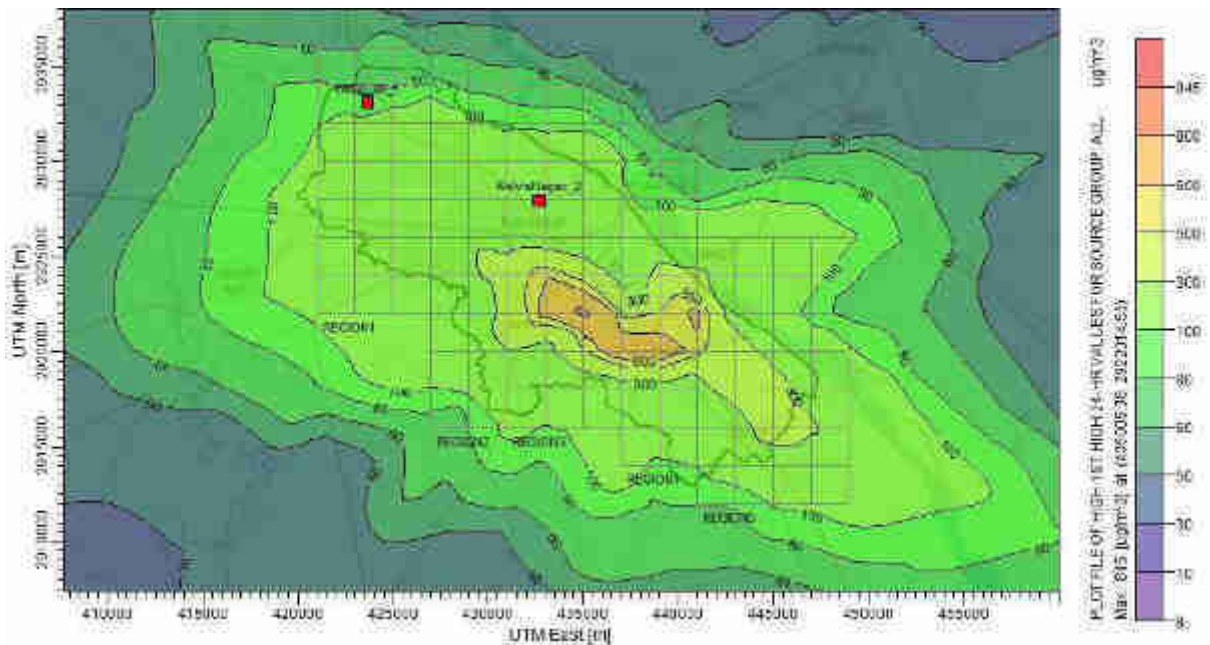
Figure 5.22: Highest 24-hour Average PM 2.5 Levels from All Sources (Scenarios 2)
