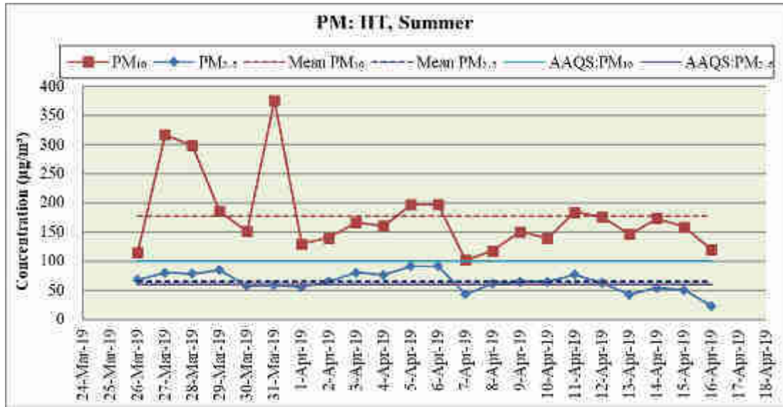
Figure 2.53: PM Concentrations at IIT for Summer Season
