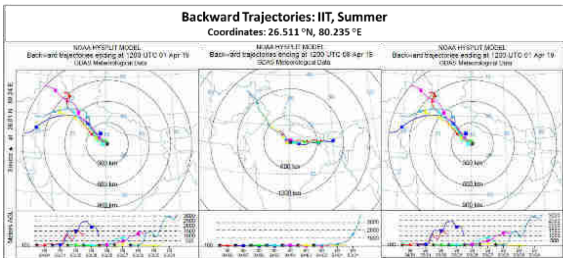
Figure 4.32: Backward trajectories at IIT for summer season
